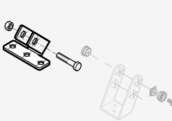
CODE. 2700107 Front frame bracket + actuator bracket accessories
