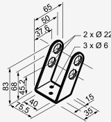
CODE. 2700124 Silver actuator support bracket
