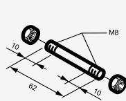
CODE. 2700102 Front pin for sunshade versions
