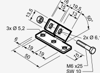
CODE. 2700064 Front bracket for window frame
